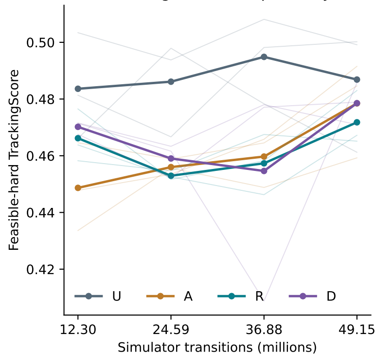
Learning curves · exploratory
